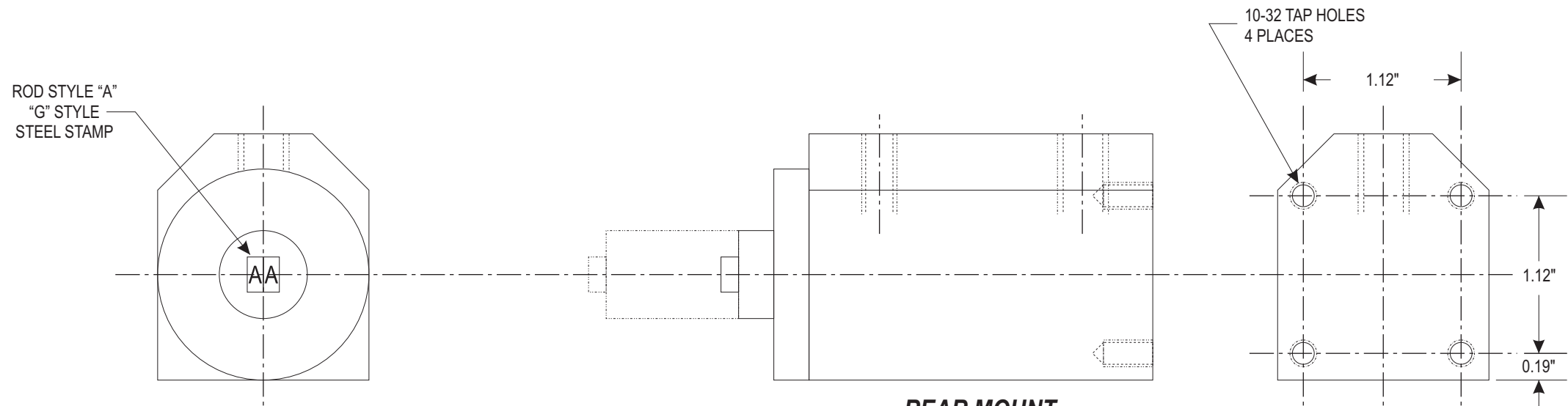
REAR MOUNT
