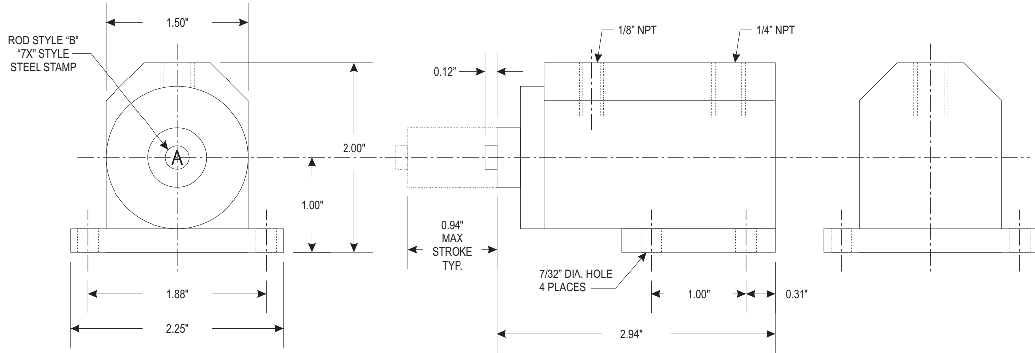
FOOT MOUNT
